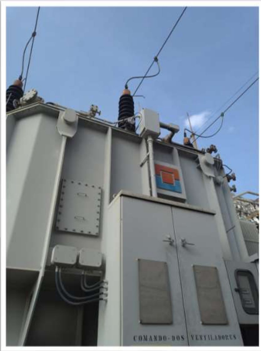
Power Transformer TUSA 138/88/13.8 Kv-20 Mva
